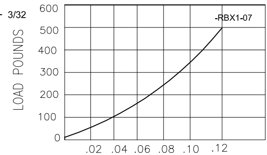
AXIAL LOAD Vs. DEFLECTION
